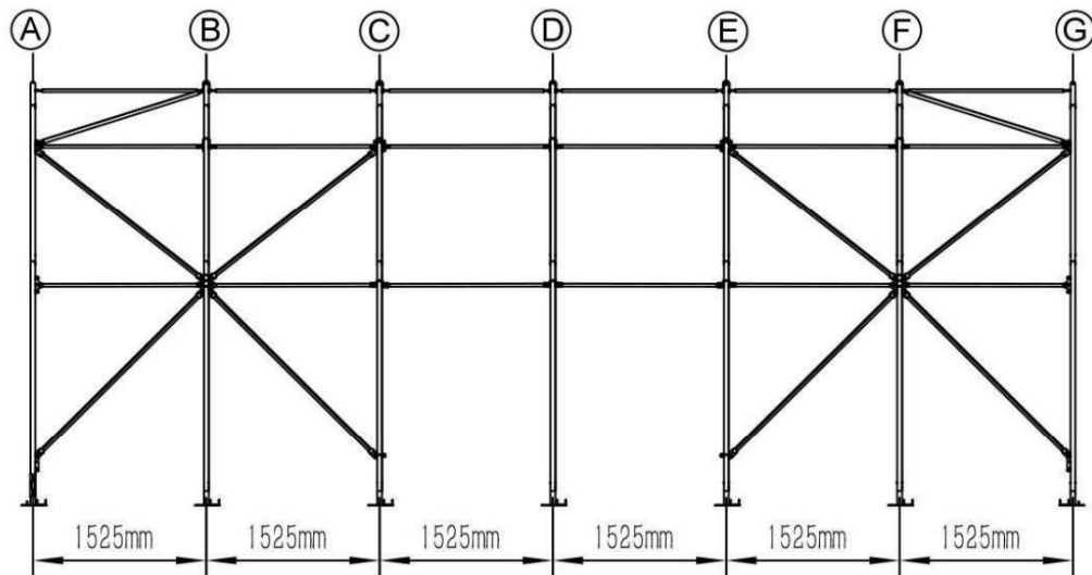
Right view
