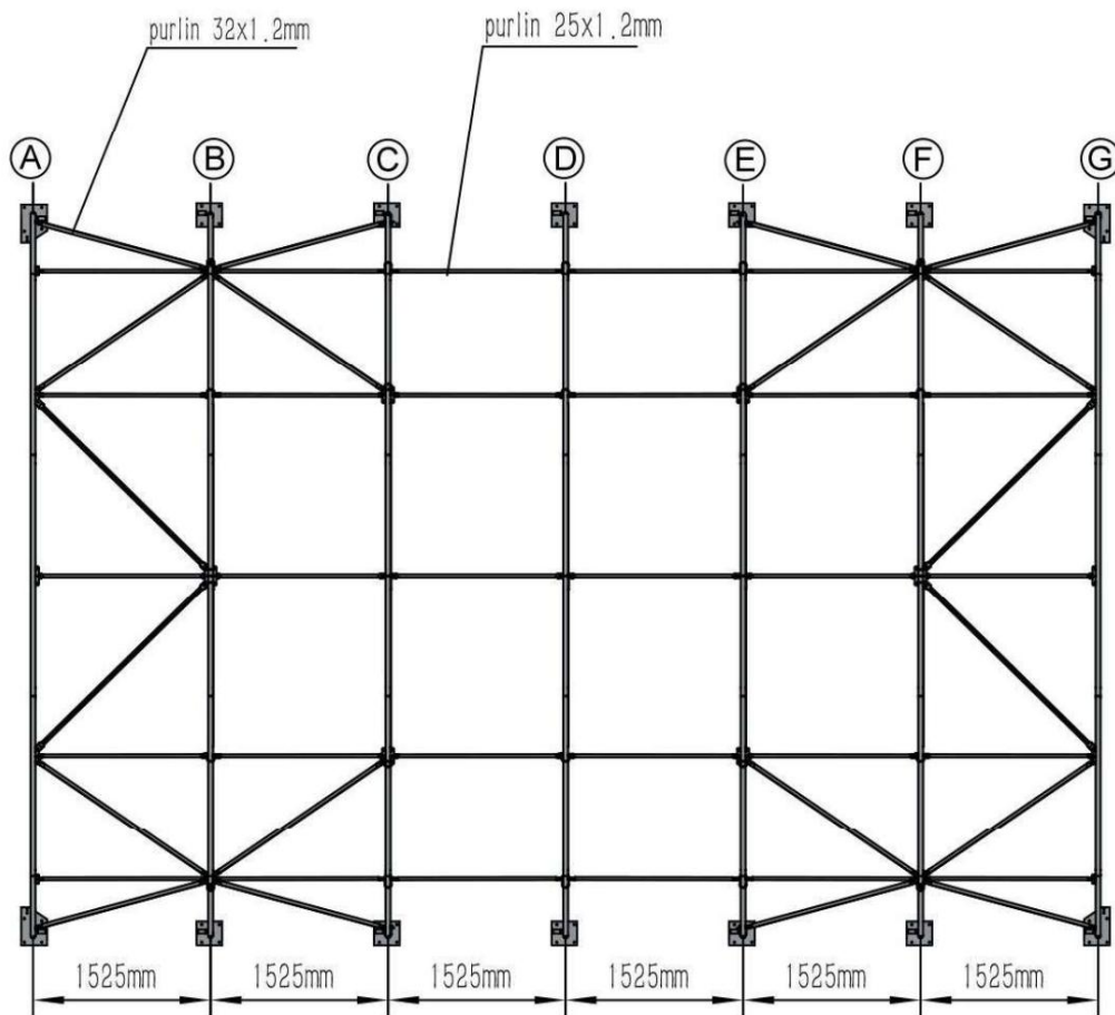
Top view
