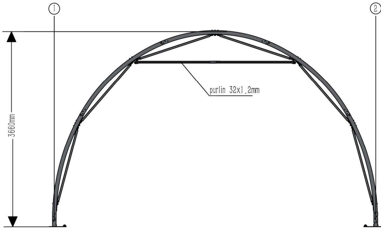
Front view
