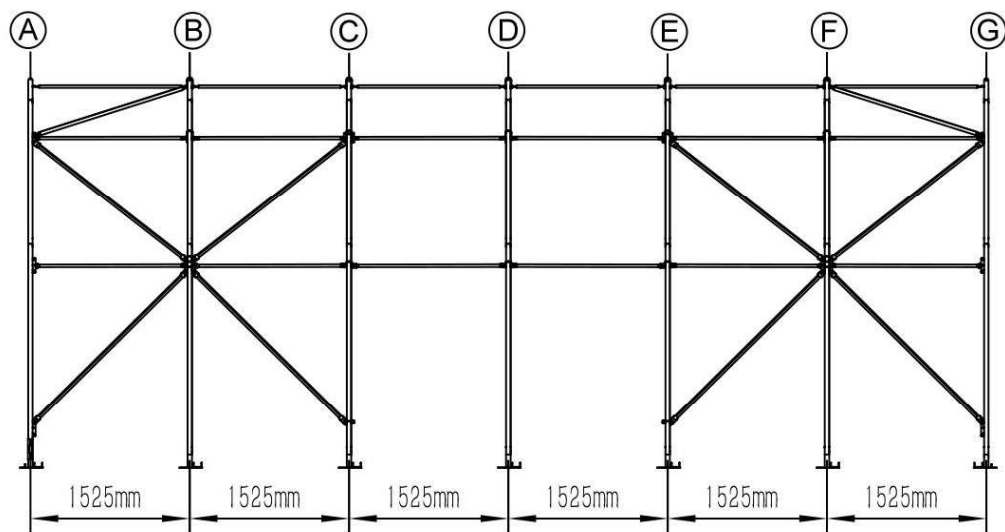
Right view
