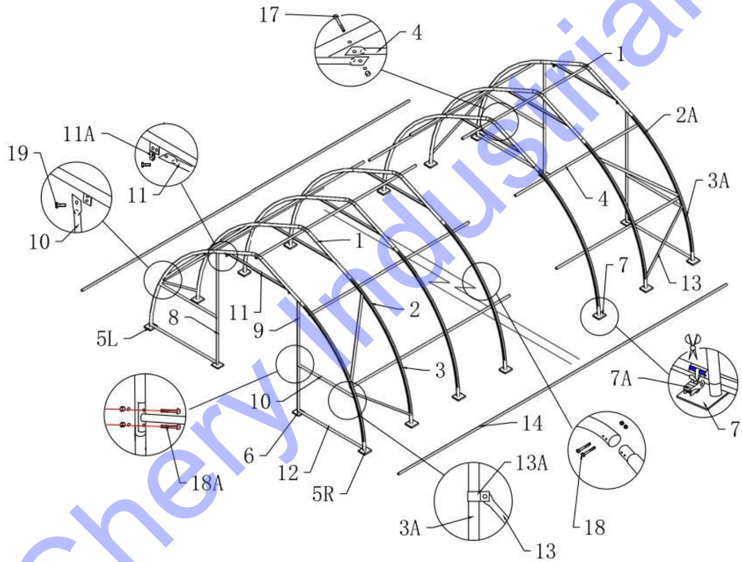
(W30'x H15' xL40'/65/'85') FRAME SKETCH Figure 3
